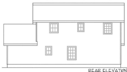
REAR ELEVATION
